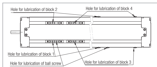
Please refer to page PS-5 for the position of the holes for lubrication for TH 90 SP 4. Fig. 11
